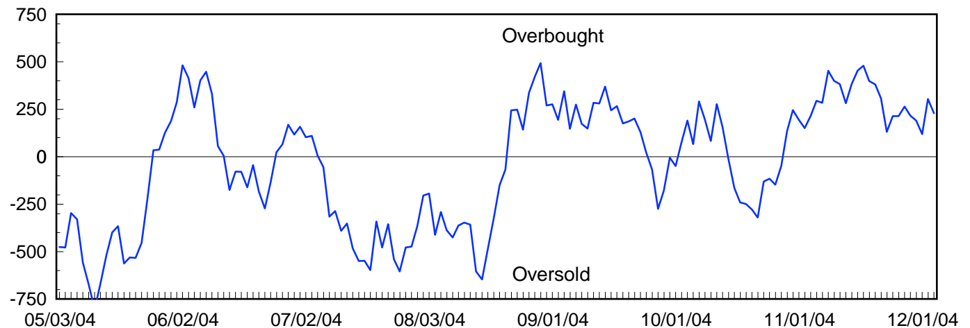
Momentum Oscillator 5
