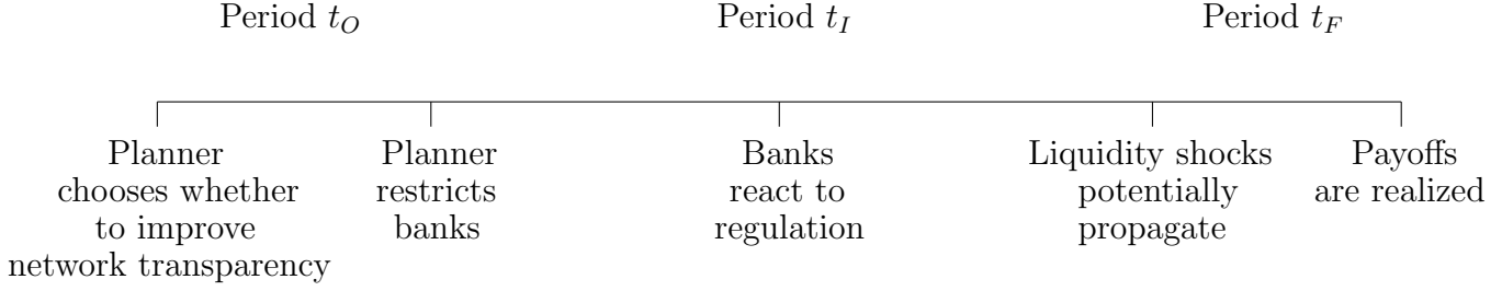
Figure 4. Model timeline
