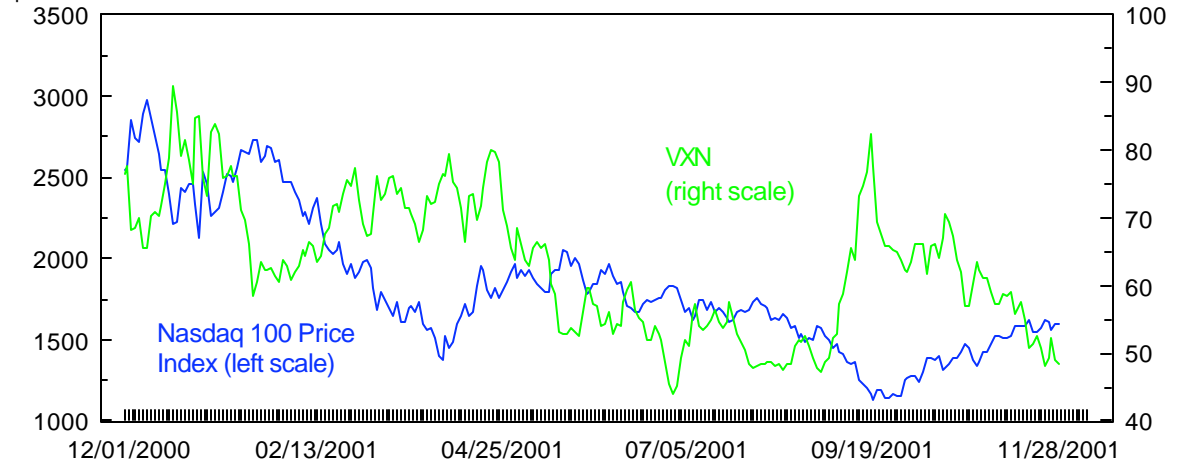
Nasdaq 100 and CBOE's NDX Volatility Index 9
