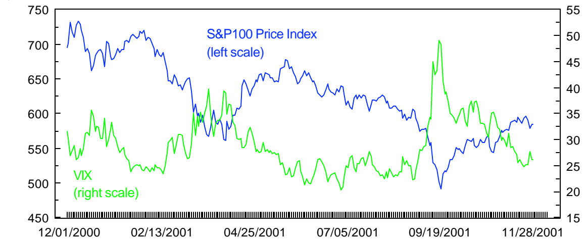
S&P100 and CBOE's OEX Volatility Index 8
