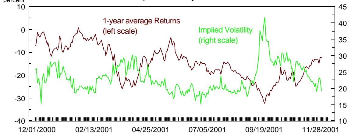
S&P500 Index Return and Implied Volatility
